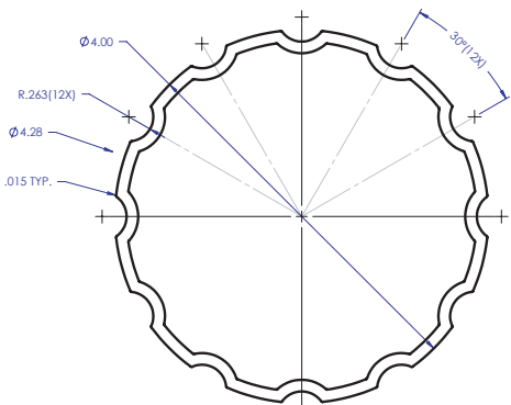
4" DIAMETER FLUTED
