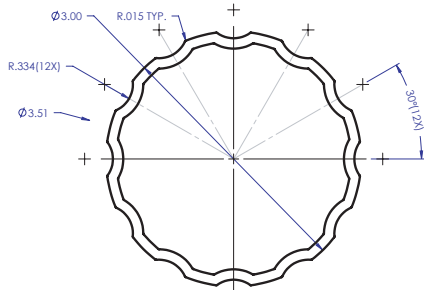
3" DIAMETER FLUTED
