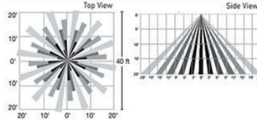
10' - 40' Mounting Height
