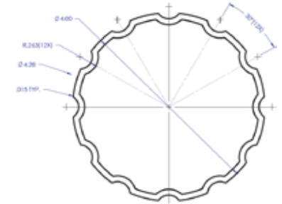
4" DIAMETER FLUTED
