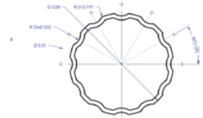
3" DIAMETER FLUTED
